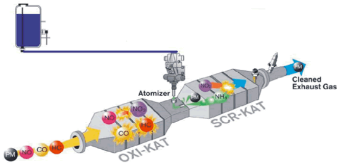
DEF / SCR System
